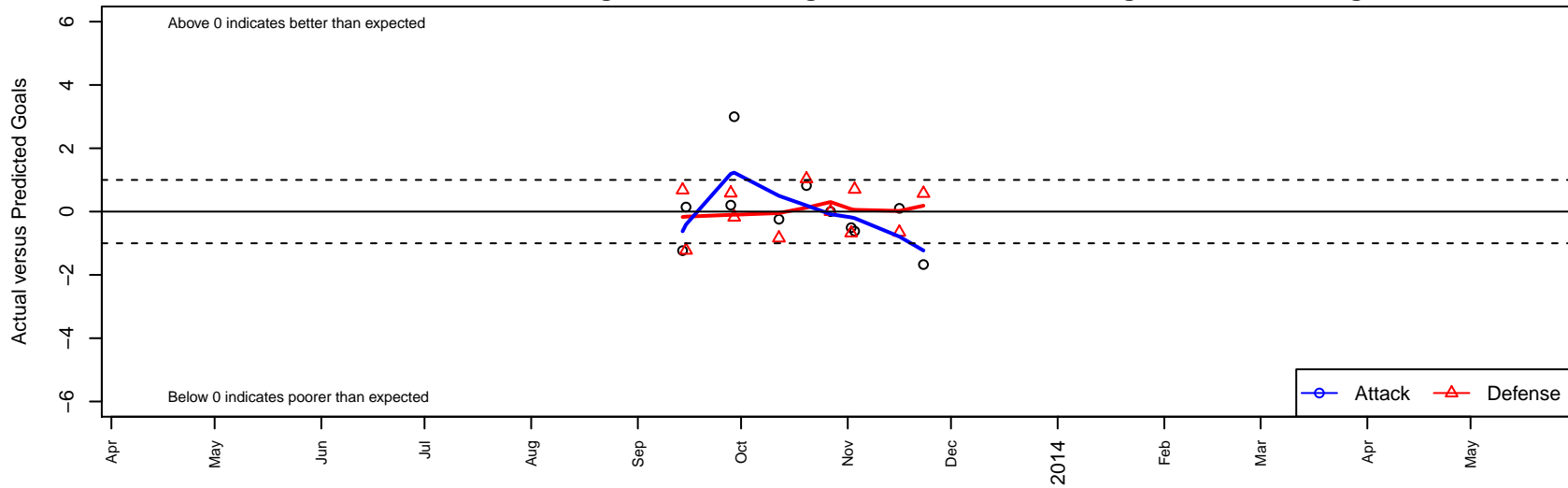
FRAM Premier 2nd B94 Dots are actual minus expected GF (blue circles) and GA (red triangles). Blue line is smoothed change in attack strength. Red is smoothed change in defense strength.
